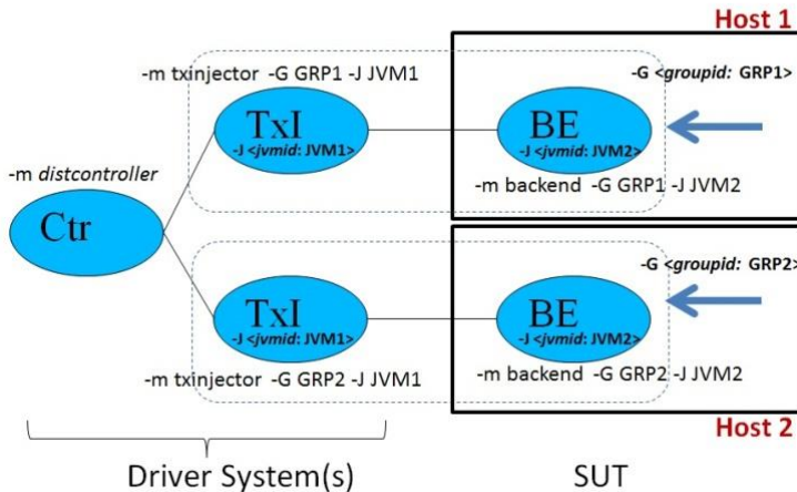
SPECjbb2013-Distributed: Backend(s) on 2 Hosts
