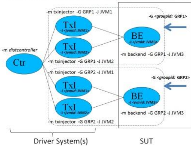
SPECjbb2013-Distributed: 2 Groups with 2 TxI/Group
