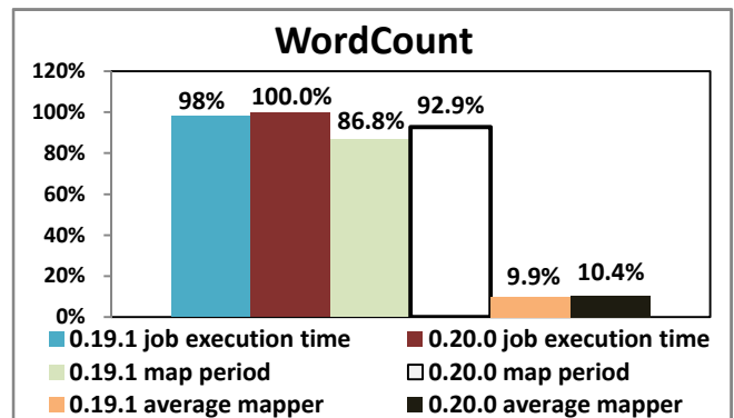
Fig. 19 normalized job execution time & map period & average mapper comparison
