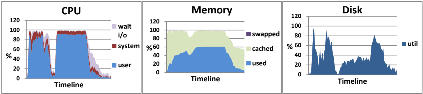
Fig. 17 NutchIndexing in the old cluster.
